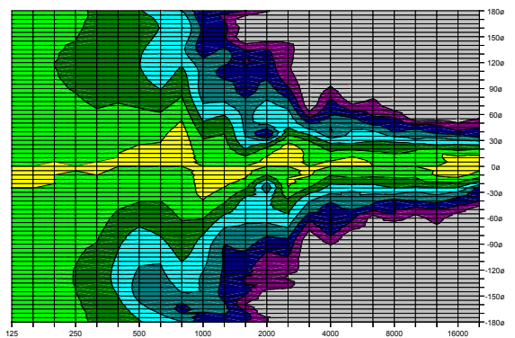
2D Directivity Plot - 90° x 60° - vertical
