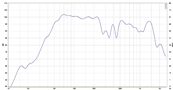
Frequency Response
